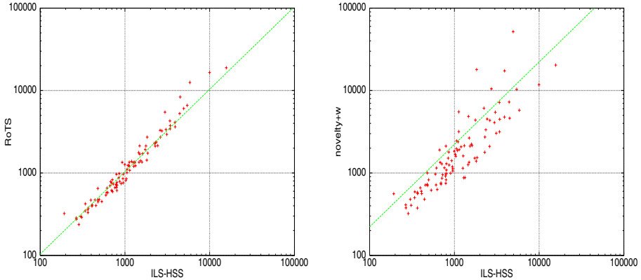
Fig. 1. Local search cost correlation between ILS-HSS and other SLS algorithms for MAX-SAT on the rnd-u (unweighted) test-set. Left: ILS-HSS vs RoTS. Right: ILS-HSS vs Novelty + /wcs+we. Along the diagonal lines, the two given algorithms require equal CPU time (compensating for differences in CPU time per search step between the algorithms).
