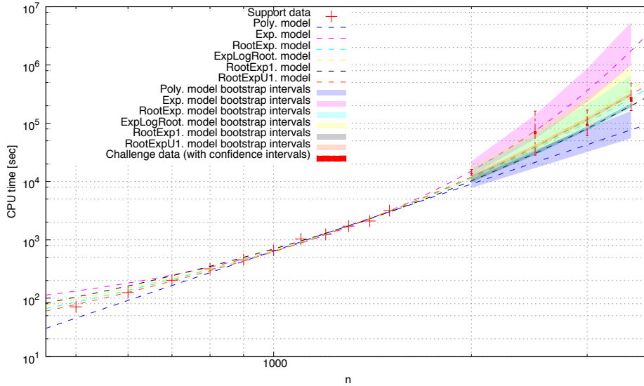
Figure 1: Fitted models of the Q90s of the running times. The models are fitted with the Q90s of the running times of Concorde-Find+Prove solving the set of RUE of 500 \leq n \leq 1500 variables, and are challenged by the Q90s of the running times of 2000 \leq n \leq 3500 variables.
