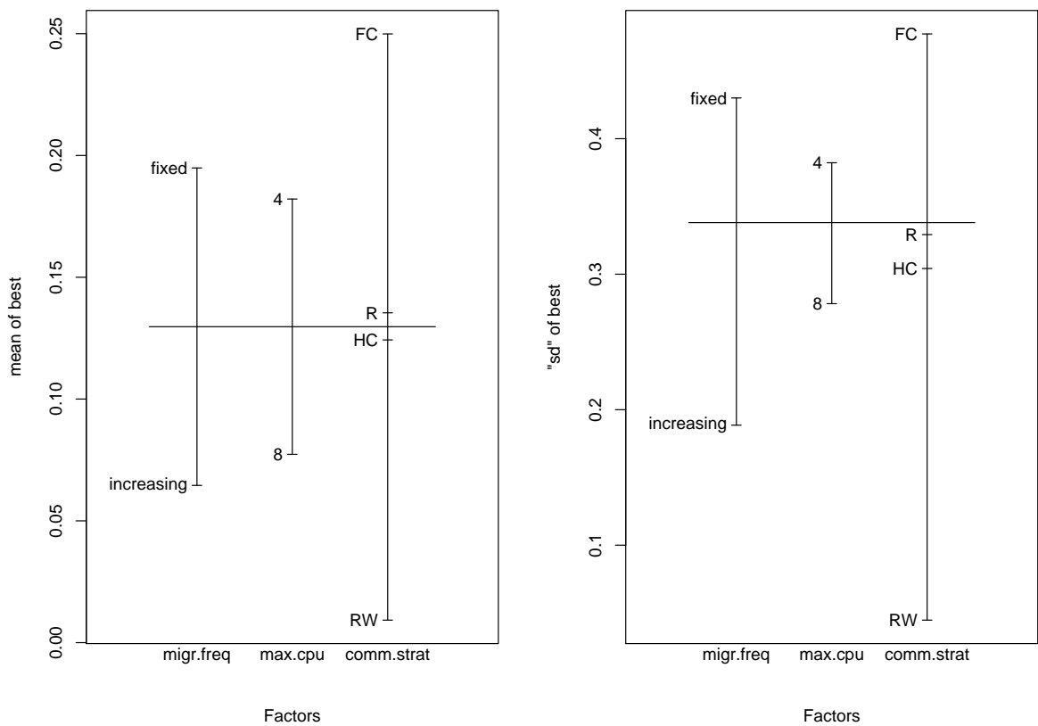
Figure 1: ANOVA design.
