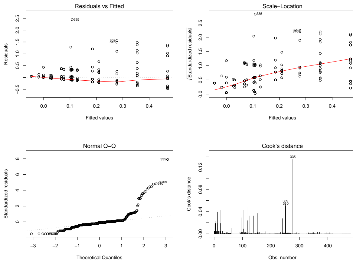
Figure 2: Diagnostic plots.
