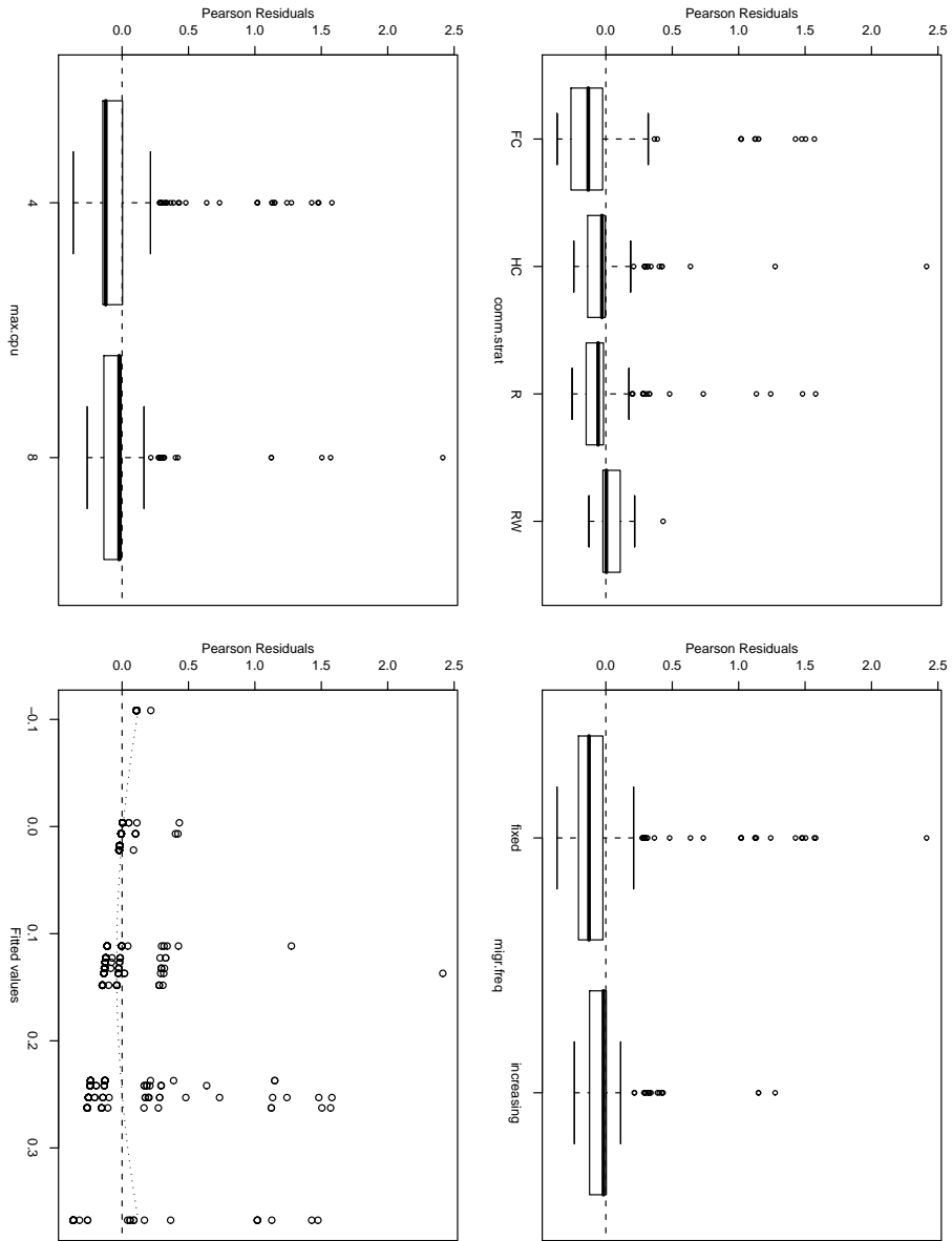
Figure 3: Diagnostic plots.
