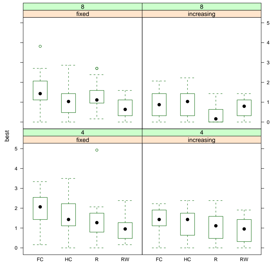
Figure 9: Boxplots.
