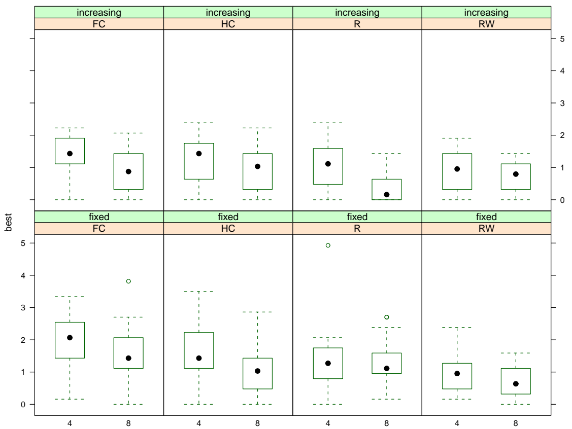
Figure 11: Boxplots.
