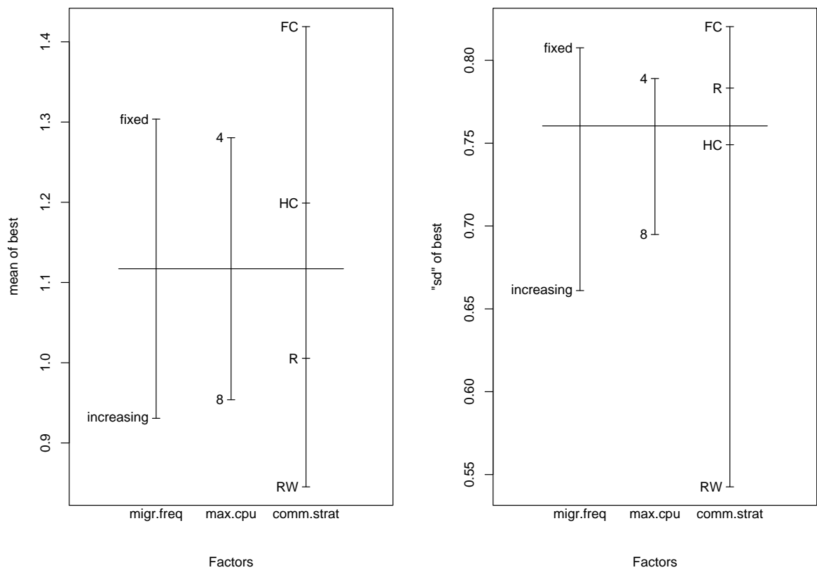
Figure 1: ANOVA design.
