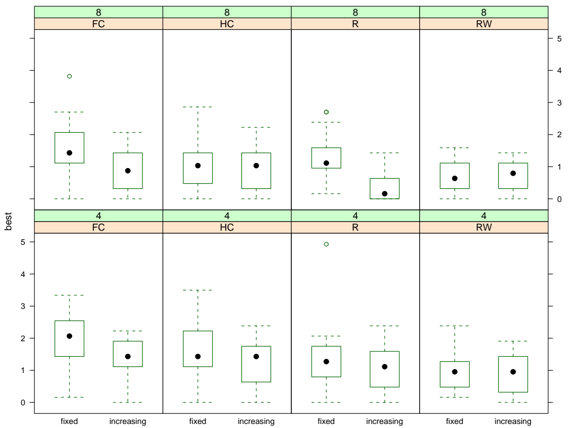
Figure 10: Boxplots.
