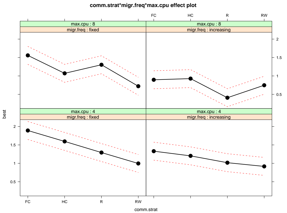
Figure 8: Third order interactions.
