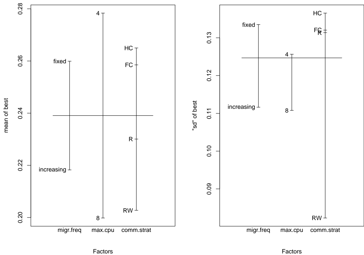
Figure 1: ANOVA design.
