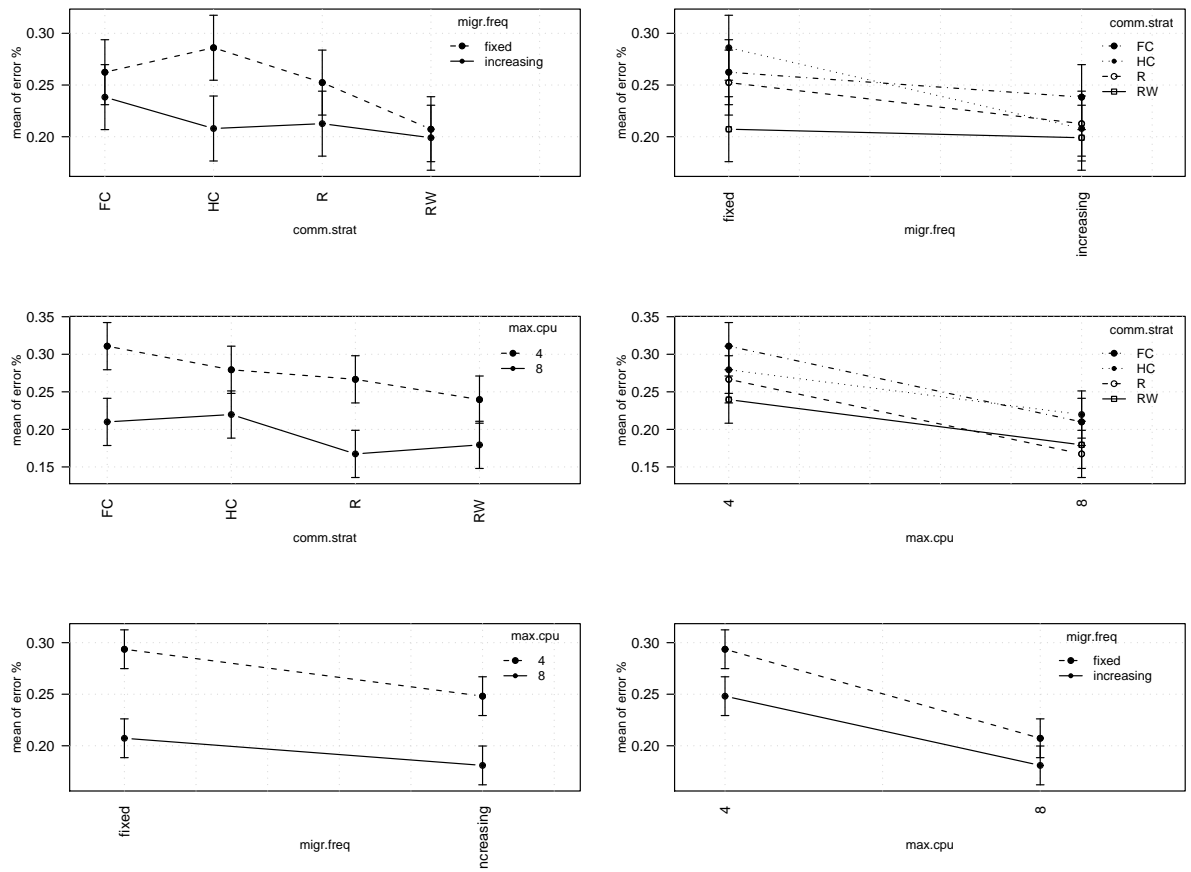
Figure 7: Second order interactions.
