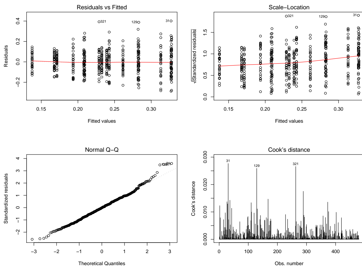
Figure 2: Diagnostic plots.
