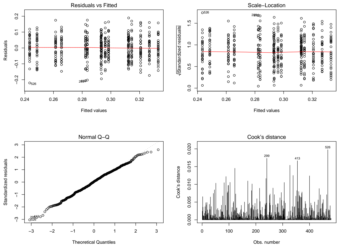
Figure 2: Diagnostic plots.
