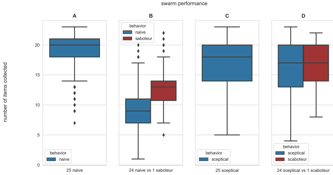
Figure 2. Box plots of the total number of items collected by each robot after 15 000 timesteps in 128 simulations per condition. Swarm size is kept constant at 25 robots in all our experiments, and we varied the swarm composition (indicated under each panel). The blue and red boxes show the results for honest and Byzantine robots, respectively. The boxes indicate the range between the data distribution’s first and third quartiles, the horizontal lines show the median, the whiskers extend in both directions to the last datapoint up to 1.5 IQR, finally, the outliers are marked black diamonds. (A-B) Naive robot’s performance has a big decrease when a single saboteur is present. (C-D) Sceptical robots are instead more resilient to the presence of a saboteur.
