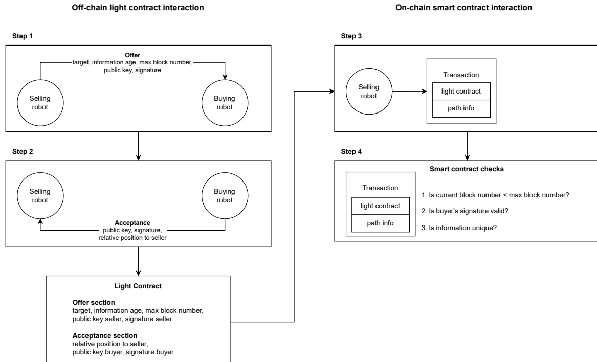
Figure 8. The process of information exchange between the selling and the buying robots comprises four steps. Step 1: A selling robot makes an offer to a buying robot. This offer includes the target (food or nest), information age, and a maximum block number which specifies when the light contract must be included in the blockchain at the latest. Step 2: If a buying robot agrees on the offer, it returns its signature of the offer and its corresponding public key. In addition, it returns its relative position to the selling robot. Both parties now possess a double-signed light contract. The light contract is an off-chain agreement between two robots that is fast to perform since it does not require a transaction on the blockchain network. Step 3: The selling robot creates a blockchain transaction that includes both the light contract and the now revealed path information to the target site in the buyer's reference frame. Step 4: The smart contract performs three security checks before it adds the transaction to the blockchain. These checks ensure that the terms of the light contract were not violated. If one of the checks fails, the transaction is discarded.
