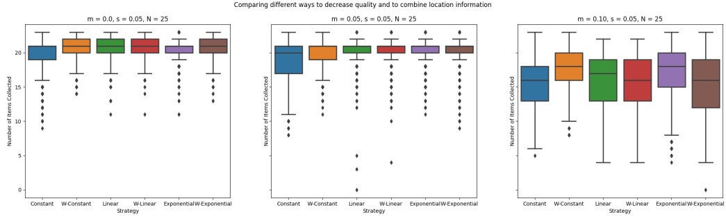
Figure S4. Comparison of different information quality and combination strategies for varying drift sampling parameter m_\mu .
