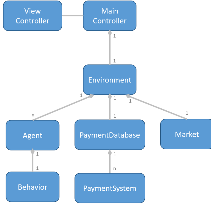
Figure S2. Simplified UML diagram describing the architecture of our multiagent simulator
