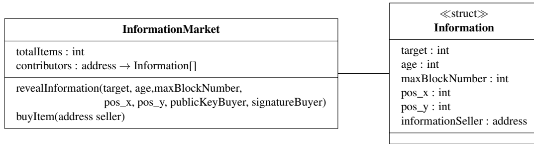
Figure 9. UML diagram of the developed smart contract. The smart contract enables the robots to buy and sell information and the market to buy items. The variable contributors is a mapping from robot addresses to a list of the Information structure. This mapping ensures that the smart contract keeps track of who sold which information to whom; the mapping is used for rewarding all contributors when the item is deposited in the nest and the market buys it.
