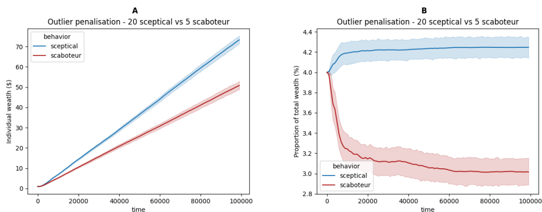
Figure S1. Average robot's wealth in a swarm of 20 sceptical and 5 scaboteur robots using the payment scheme of outlier penalisation (without staking) in 32 simulations. The transparent shades show the 95% confidence interval. (A) The absolute wealth of scaboteurs increases at a smaller rate than the one of honest sceptical robots; however the wealth of both types of robots constantly increases. (B) The proportion of total wealth rapidly converges to a relatively stable situation where scaboteurs have a smaller proportion of wealth than honest robots; however each scaboteur still collects about 3% of the total wealth. These results motivated the introduction of a new payment scheme, outlier penalisation with staking.
