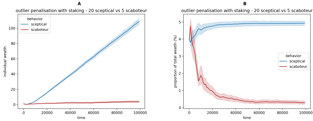
Figure 5. Average robot's wealth in a swarm of 20 sceptical and 5 scaboteur robots using the outlier penalisation with staking payment scheme in 32 simulations. The transparent shades show the 95% confidence interval. (A) The absolute wealth of honest sceptical robots constantly increases at a high pace compared with the scaboteurs that remains with relatively low, almost null, wealth. (B) The proportion of total wealth rapidly converges to a relatively stable situation where wealth is mainly distributed among honest robots, approximately equally.
