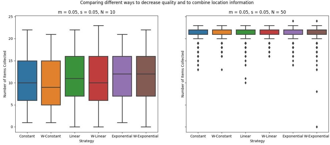
Figure S3. Comparison of different information quality and combination strategies for varying population sizes.
