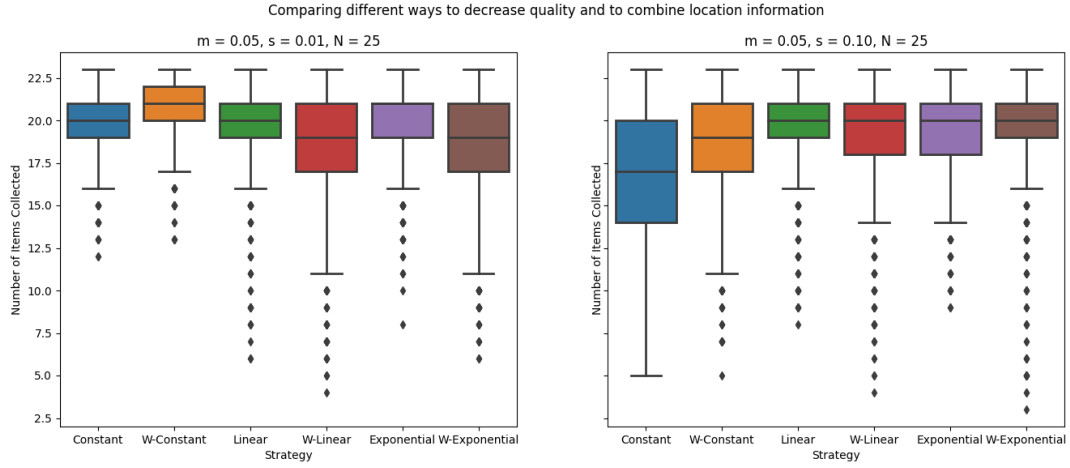
Figure S5. Comparison of different information quality and combination strategies for varying drift sampling parameter s_\mu .
