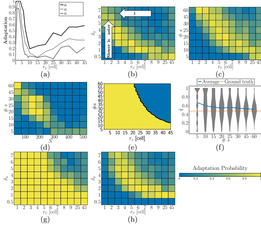
Fig. 2: (a,b,c) Less communication leads to higher adaptation probability. This effect happens only when recruitment is slow, i.e., in the top part of panels (b,c), for high sampling times \tau_s = s \delta_s , which can be caused by (b) large times between samples \delta_s (with fixed s = 15 ) or (c) high numbers of samples s (with fixed \delta_s = 1 ). (b-c) When communication is limited, slower sampling time leads to higher probability of adapting. (d) The same two effects can be observed for fixed communication range ( r_c \approx 12.5 cm for c = 3 ) and increasing robot density, which we control by modifying the swarm size N in an environment with a fixed size; (e) the ODE model (Eq. (1)) predicts qualitatively similar to results as seen in simulations ( N = 50 , \kappa = 0.9 , k = 4 \times 10^{-6} ); (f) sampling times \tau_s influence the noise, because accuracy increases when robots collect more samples s , or reduces sample correlations with larger times \delta_s in-between samples; (g) when estimation noise is independent of sampling and low ( \sigma = 0 ) the slower-is-faster effect disappears; (h) when estimation noise is independent of sampling and high ( \sigma = 0.1 ) both effects are present; if not specified, swarm size N = 50 , difficulty \kappa = 0.9 , 30 simulations each; colour-maps show probability to adapt.
