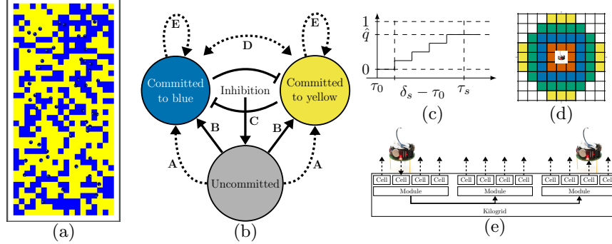
Fig. 1: (a) collective perception scenario for simulated Kilogrid in ARGoS (simulation code, see [2]), swarm of N = 50 Kilobots (small circles); (b) robots controlled by finite state machine with n + 1 states (here n = 2 ), transitions: self-sourced (dashed arrows) or social (solid arrows) evidence; uncommitted \rightarrow commit through (A) discovery or (B) recruitment; committed robots change state by: (C) cross-inhibition, (D) direct switching, or (E) stay; (c) once recruited, robots gradually increase com. probability w for sampling time \tau_s = s \delta_s , s samples every \delta_s seconds; (d) robot-to-robot com. is virtualised using Kilogrid; (e) focal Kilogrid module receives Kilobot message and sends to all cells within com. range (prop. to param. c ; com. range r_c , c = \{2, 3, 4, 5\} ).
