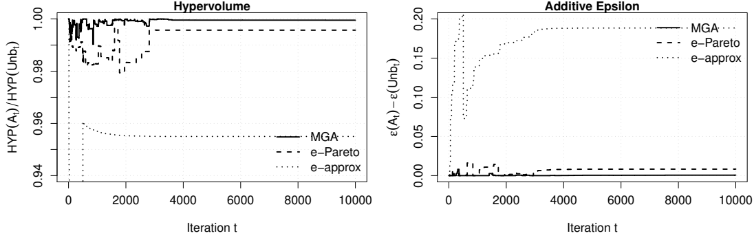
Fig. 2. Small PF (2D) N = 10
