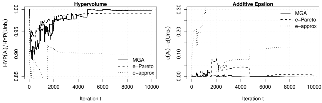
Fig. 3. Small PF (3D) N = 10
