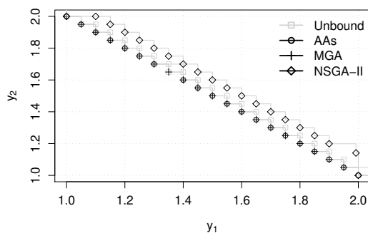
Fig. 6. NSGA-II may \prec -deteriorate over time, N = 20
