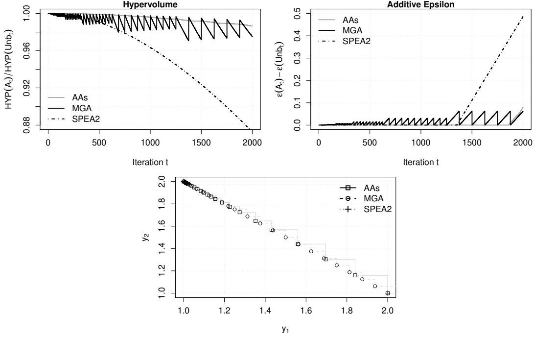
Fig. 5. Increasing extremes (2D) affects SPEA2 performance, N = 20
