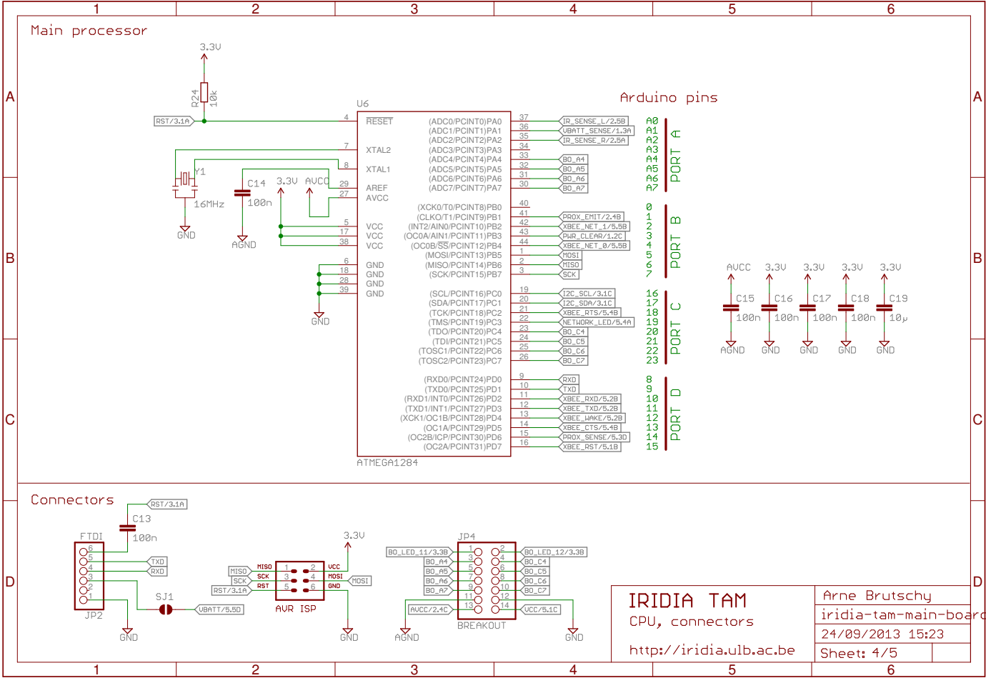
Figure B.4: Circuit schematics for the main processor and supporting connectors
