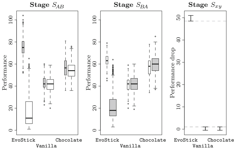
Fig. 3 FORAGING. Left and center: Performance in the two stages—the higher, the better. Right: Performance drop, aggregated across the two stages—the lower, the better. See caption of Fig. 2 for a detailed description of the figures
