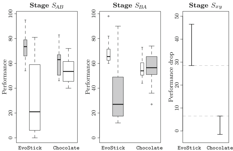
Fig. 6 Results for FORAGING. See caption of Fig. 5 for a detailed description
