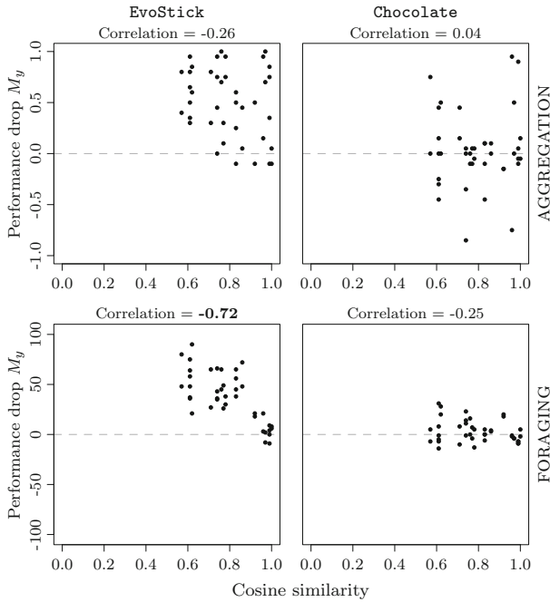
Fig. 9 Pearson correlation between performance drop and cosine similarity between models used for design and evaluation. See caption of Fig. 7 for more details
