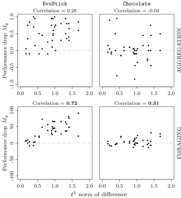
Fig. 8 Pearson correlation between performance drop and \ell^1 norm of the difference between models used for design and evaluation. See caption of Fig. 7 for more details
