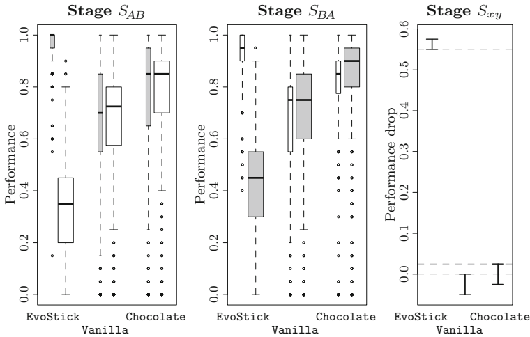
Fig. 2 AGGREGATION. Left and center: Performance in each stage—the higher, the better. Narrow boxes represent the performance assessed on the design model; wide boxes represent the performance assessed on the pseudo-reality. Gray boxes represent performance assessed on M_A ; white boxes represent performance assessed on M_B . Right: Performance drop, aggregated across the two stages—the lower, the better. The segments represent the upper and lower bounds on the performance drop experienced in pseudo-reality—bounds are computed using Wilcoxon statistics, at 95% confidence
