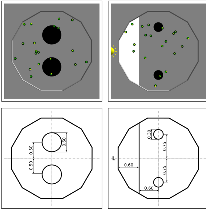
Fig. 1 ARGo3 representations and technical diagrams of the arenas: AGGREGATION (left) and FORAGING (right). Measures are expressed in meters. For FORAGING, a light is placed behind the nest so that it is visible from everywhere in the arena
