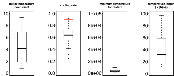
Figure 5: Distribution of the parameter values obtained after the tuning phase for the BIN algorithm, relatively to the allowed range. In red, the default value of each parameter.
