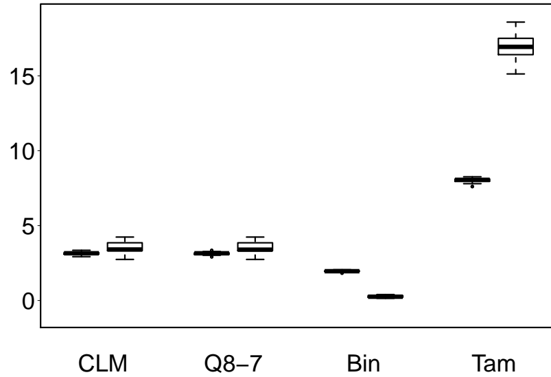
Figure 1: Relative Percentage Deviation from the best-known solutions obtained by the default versions of the four SA algorithms compared. For each algorithm there are two results reported, for random instances (plot on the left) and structured instances (on the right).
