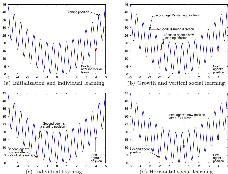
Figure 1: The incremental particle swarm-guided local search algorithm at work. In Figure (a), an initial particle is randomly placed in the search space. Immediately after, the first round of individual learning (local search) is run, moving the particle to, or close to, a local minimum. This is followed by a horizontal learning round (a normal PSO move) that does not have any effect in a swarm of one particle (the particles' velocity are initialized to zero). In Figure (b), the size of the population is increased. The vertical social learning rule (Eq. 3) is used to place the new particle in the search space. In Figure (c), the second iteration of the algorithm begins by running a round of individual learning. In Figure (d), through a round of horizontal learning, particles can move and discover more promising areas of the search space. The algorithm continues intertwining individual and social learning procedures until a stopping criterion is satisfied.
