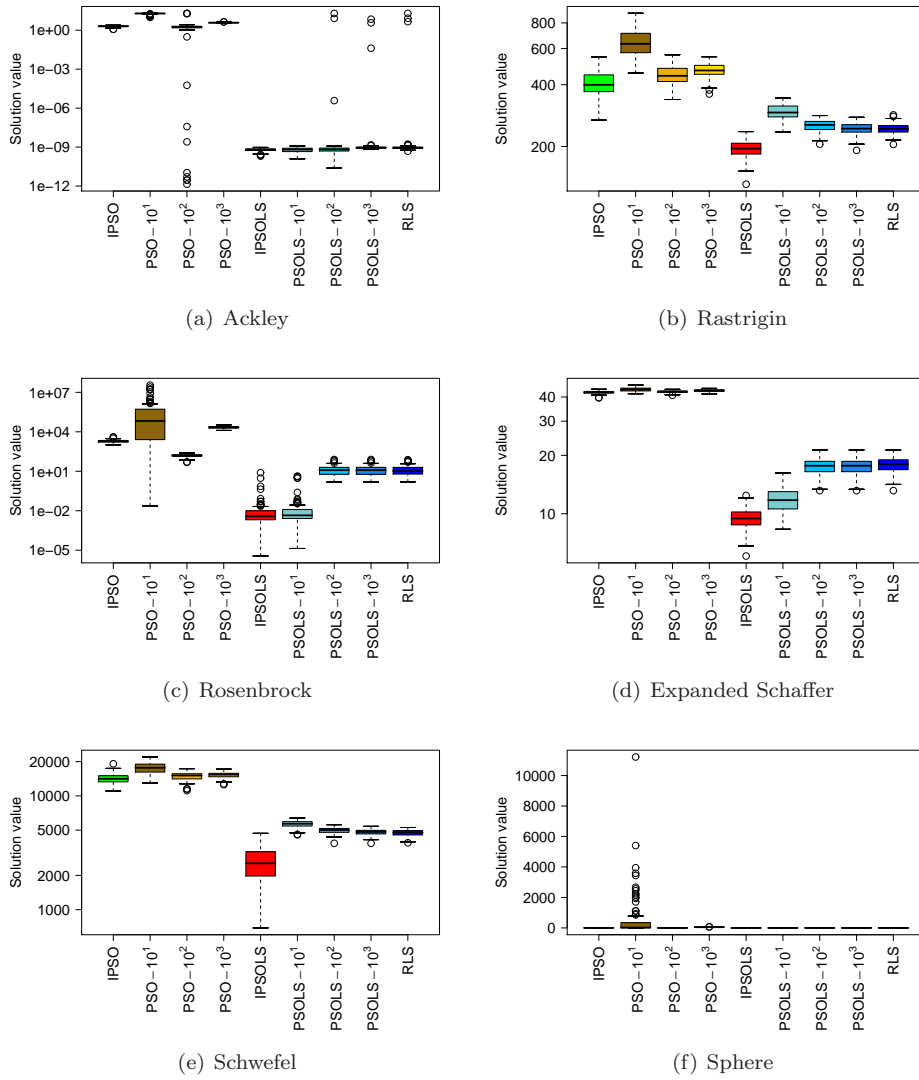
Figure 2: Boxplots showing the distribution of the solution quality obtained by the compared algorithms after 10^6 function evaluations. These results correspond to the case in which all particle swarm-based algorithms used a ring topology. The numbers next to the labels indicate the population size used.
