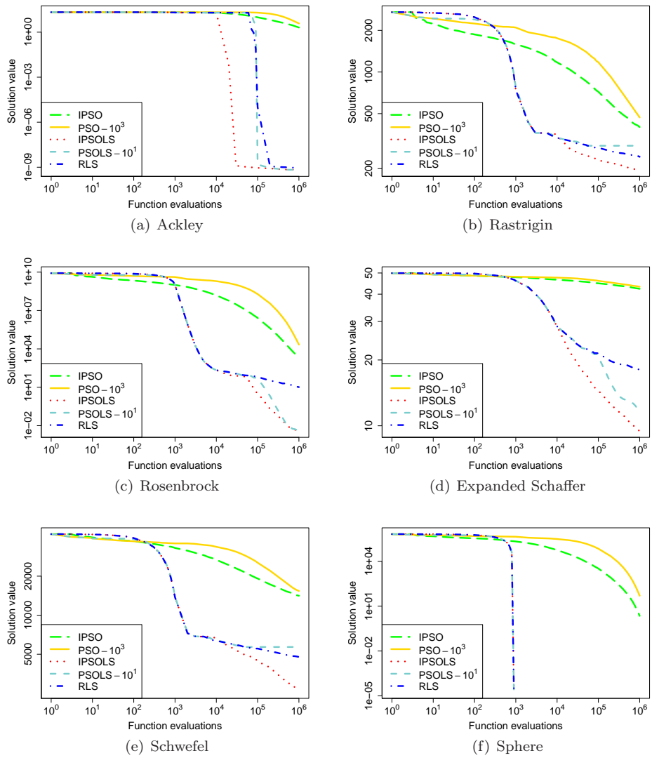
Figure 3: Development of the solution quality over time (median values). These results correspond to the case in which all particle swarm-based algorithms used a ring topology. The numbers next to the labels indicate the population size used.
