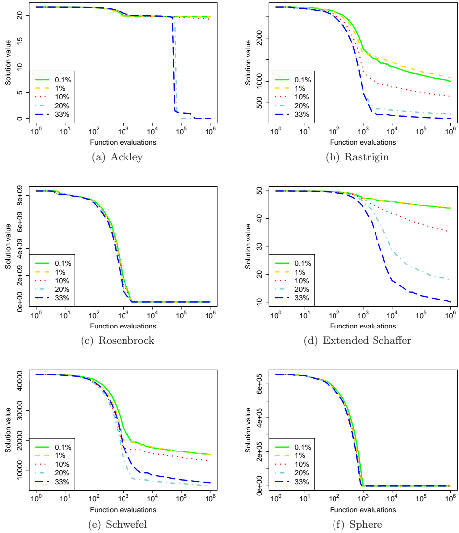
Figure 4: Development of the solution quality over time (median values) for different local search step sizes using RLS.
