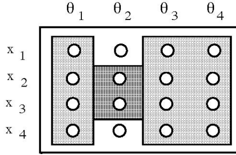
Figure 1: Ballooning of the bbm m(x_2 \cup x_3 \upharpoonright \theta_2) (dark area) onto X \times \Theta (shaded area). The white dots correspond to the 16 elements of X \times \Theta .
