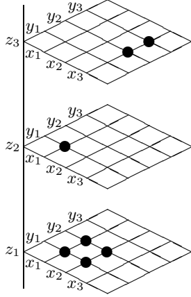
Figure 1: Example of a Z-layered rectangle, dots indicate its elements.
