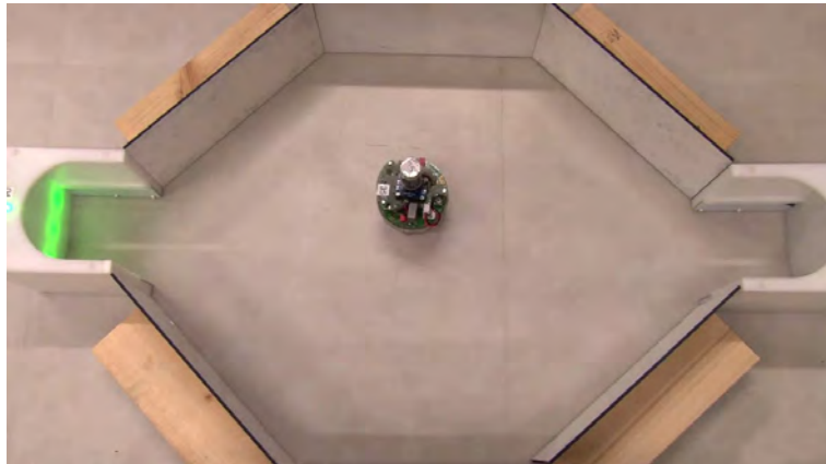
Figure 5.8: Snapshot recorded during the first TAM reliability experiment, where a single e-puck robot has to continuously perform two stationary atomic tasks. In the situation shown, the e-puck has recently completed the blue task represented by the TAM on the right side. The TAM on the left side is now announcing a green task, which is perceived by the e-puck.
