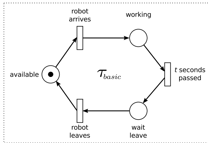
Figure 4.3: Basic low-level Petri net model of an atomic task \mathcal{T}_{basic} with three states. The state of the task changes depending on external events.
