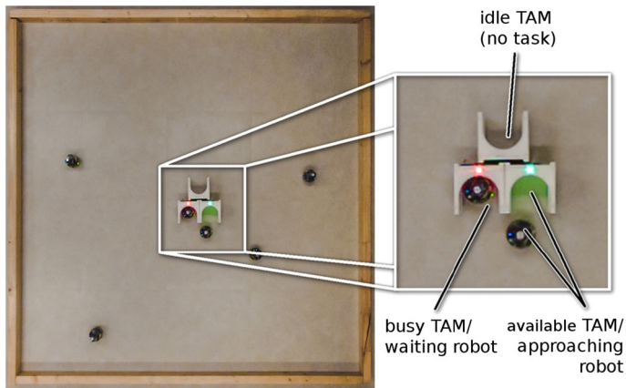
Fig. 11 Snapshot of the single-instance demonstration, taken with an overhead camera in the same situation as shown in Fig. 10a. The arena is a 4 m 2 square. A single instance of the task \tau_{\text{response}} , abstracted using three TAMs, is placed in the center of the arena. We use 6 e-puck robots
