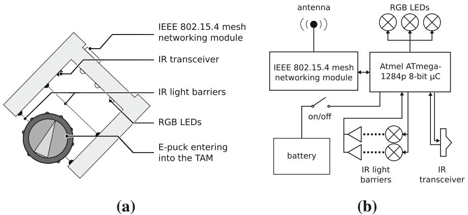
Fig. 3 a Schematic drawing of the TAM. b Block diagram showing the functional components of the TAM
