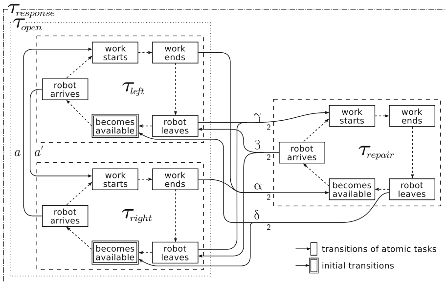
Fig. 9 Low-level Petri net model of the example task \tau_{response} (reduced version without places) (see Footnote 6). Please note that, as the initial marking cannot be visualized in the reduced version, we denote transitions that can fire at the start of the demonstration using a double border. The weight of all edges is 1 unless indicated otherwise. Edges that are internal to the functioning of an individual TAM are represented using dashed lines . Edges labeled a and a' model the concurrent interrelationship: a robot that is ready to work on \tau_{left} can start working once a robot arrives to work on \tau_{right} (and vice versa). Edges labeled using Greek letters model the sequential interrelationship: once \tau_{left} and \tau_{right} have been completed, \tau_{repair} becomes available (edge \alpha ); a robot that arrives to work on \tau_{repair} allows the robots in \tau_{right} and \tau_{left} to leave (edge \beta ); once these robots have left, work can start on \tau_{repair} (edge \gamma ); once work on \tau_{repair} finishes and the robot leaves, \tau_{right} and \tau_{left} can become available anew (edge \delta ). Dotted/dashed boxes indicate task boundaries
