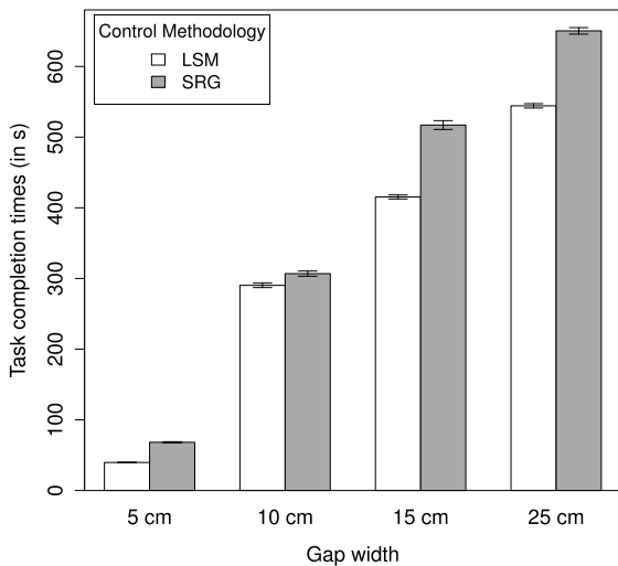
Fig. 9. Results of the experiments carried out to isolate the benefits of group selection based on location (LSM) vs. random group selection (SRG). The results presented are task completion times of the two strategies for all the four environments considered. Note that the group selection and formation times have been omitted for LSM and SRG in order to facilitate a meaningful comparison. Standard deviations are added to the bars.
