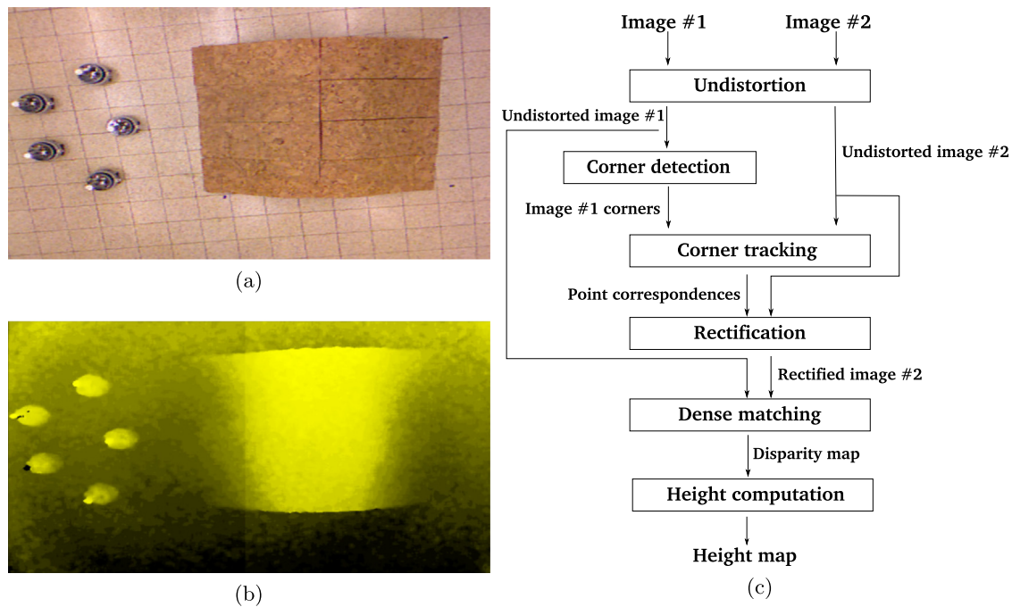
Fig. 10. Computing height maps using images retrieved from a monocular camera. (a) A 640 \times 480 image acquired by the eye-bot. (b) A representation of the computed disparity map in which brighter pixels denote greater motion and lesser distance from the camera. (c) A flowchart showing the computation of height maps based on a pair of stereo images. The result is a two-dimensional matrix with the elevation in cm for each pixel.
