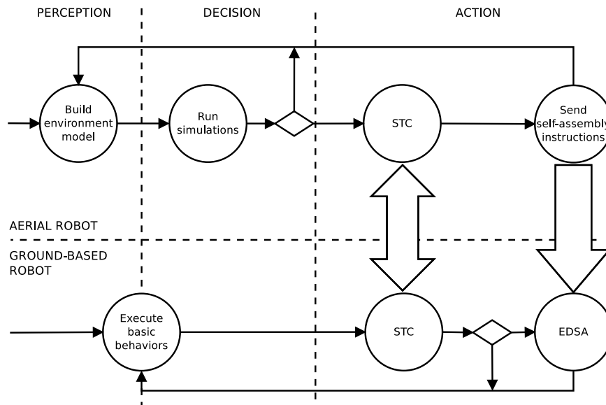
Fig. 2. An overview of supervised morphogenesis. Each circle represents a control state related to perception, decision or action taken by the heterogeneous team. Basic behaviors (such as phototaxis and obstacle avoidance) depend on the actual task and may include perception and decision-related activities that do not require aerial supervision. The vertical arrows indicate the occurrence and directionality of interactions between the robot types. STC: spatially targeted communication, EDSA: enhanced directional self-assembly.
