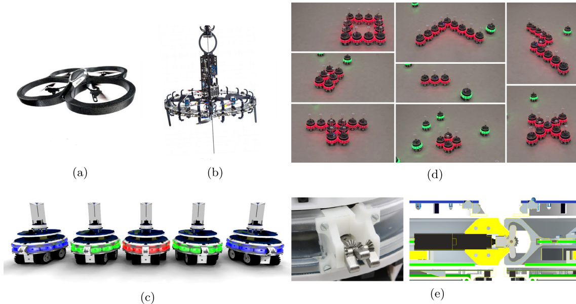
Fig. 1. The robot platforms used in this work. (a) The AR.Drone. (b) The eye-bot. (c) Five foot-bots capable of self-assembly with their LEDs illuminated in different RGB colors. (d) A photo montage showing example morphologies that can be formed by multiple foot-bots. (e) The three-fingered connection device of the foot-bot before and after insertion into the passive docking ring of another robot.
