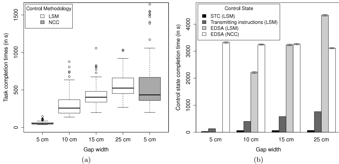
Fig. 8. Results confirming how supervision from the eye-bot (i.e., LSM) lowers the task completion times of the overall system when compared to a control strategy (i.e., NCC) that does not rely on aerial supervision. (a) Box-and-whisker plot showing task completion times (in seconds) of LSM in four different environments. For the NCC methodology, results of only one environment are plotted as they do not differ significantly from each other. (b) Bar-plot showing a breakdown of the time spent by the foot-bots executing different control states. Bars are decorated with the standard deviation, except for the control state “transmitting instructions” that is bound to constant time for each transmitted SWARMORPH-script (i.e., the gap width).
