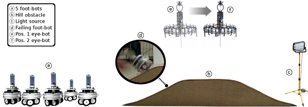
Fig. 4. The experimental setup of the hill-crossing task. Five foot-bots are shown in the deployment area. A light source representing the destination area is shown on the right. A hill obstacle that cannot be crossed by an individual foot-bot is shown between the areas. Visualized are also two positions above the hill obstacle the eye-bot considers when using its monocular vision system.
