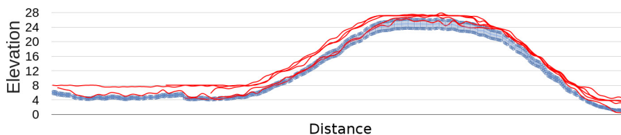
Fig. 11. Mean elevation of height profiles acquired by the eye-bot from 10 different height maps. Graphs in red result from computation based on stereo images while data retrieved from the Kinect sensor is shown in blue. (For interpretation of the references to color in this figure legend, the reader is referred to the web version of this article.)
