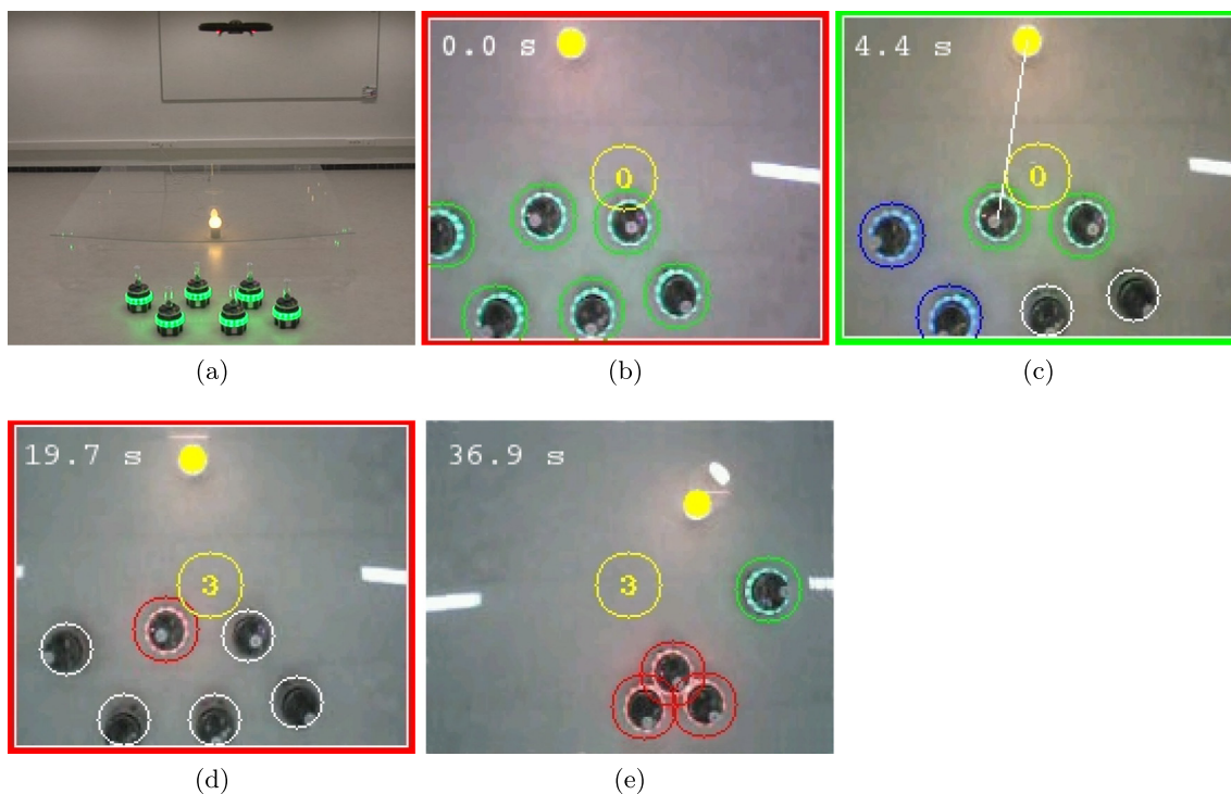
Fig. 3. The experimental setup of case study 1. (a) The robot team is composed of one AR.Drone and six foot-bots. A light source is placed on the ground. (b–d) are frames taken from the AR.Drone camera when executing STC. Border colors visualize transmitted messages; the number in the center of each frame shows the size of the target morphology resulting from the simulations run by the AR.Drone. (e) shows the target morphology formed using EDSA. The times shown in (b–e) correspond to the clock time starting the execution of STC. For safety reasons, a transparent plexiglass platform is installed at 40 cm height in the area of the light source in order to shield the foot-bots from the AR.Drone executing emergency landing behaviors. (For interpretation of the references to color in this figure legend, the reader is referred to the web version of this article.)
