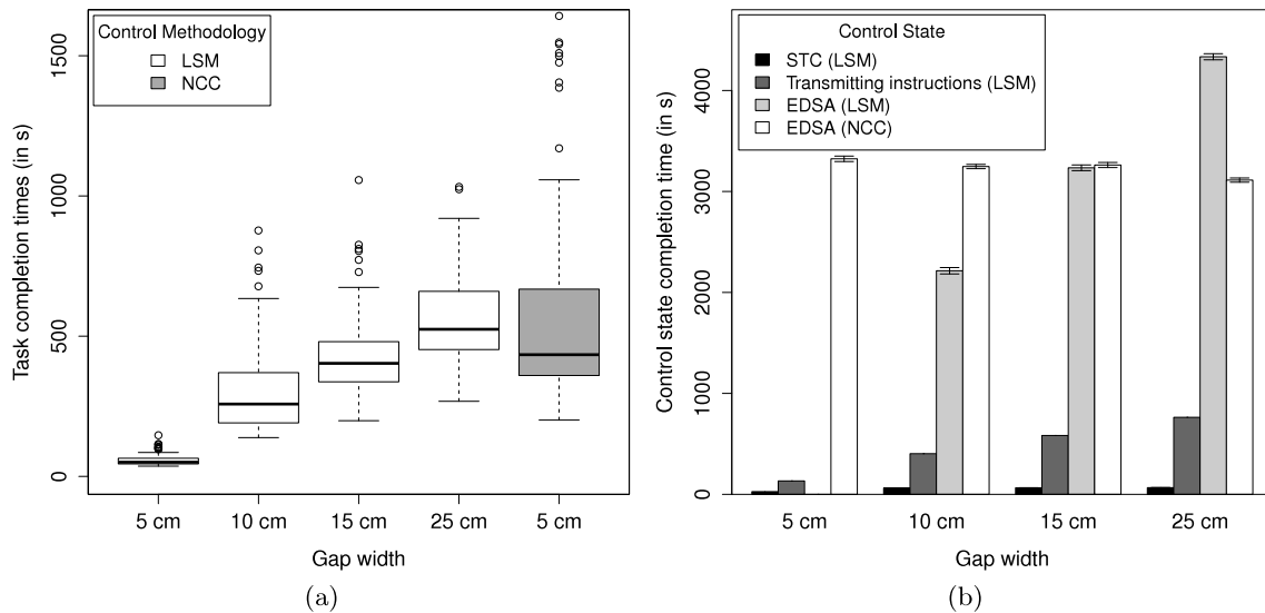
Fig. 8. Results confirming how supervision from the eye-bot (i.e., LSM) lowers the task completion times of the overall system when compared to a control strategy (i.e., NCC) that does not rely on aerial supervision. (a) Box-and-whisker plot showing task completion times (in seconds) of LSM in four different environments. For the NCC methodology, results of only one environment are plotted as they do not differ significantly from each other. (b) Bar-plot showing a breakdown of the time spent by the foot-bots executing different control states. Bars are decorated with the standard deviation, except for the control state “transmitting instructions” that is bound to constant time for each transmitted SWARMORPH-script (i.e., the gap width).
