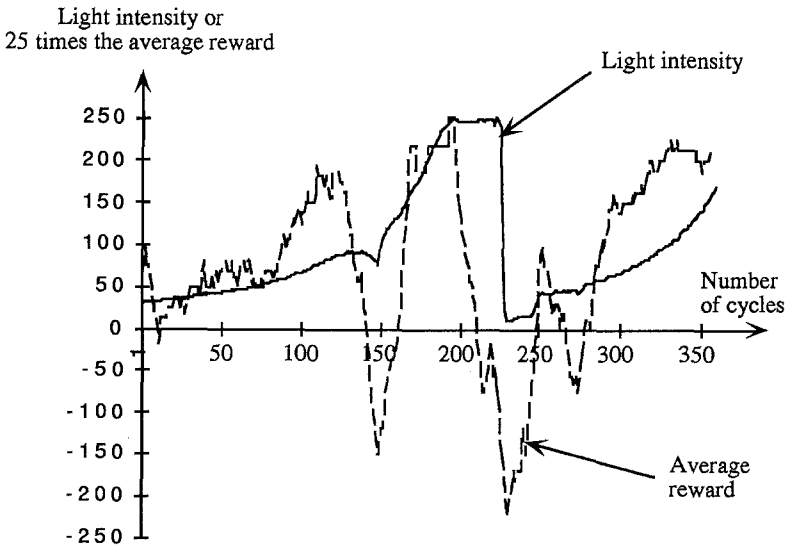
Figure 19. System performance (light intensity) and average reward (multiplied by 25 to ease visual comparison) for the reward-the-result training policy.
