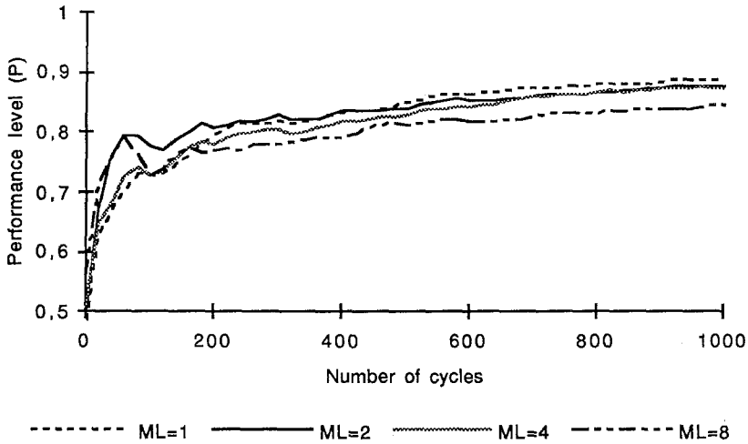
Figure 12. Learning to follow a light source (the playing behavior). A comparison of different ML lengths, using the rewards and punishments training policy. Averages on twenty runs.
