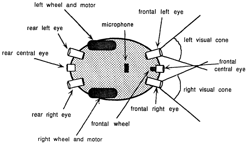
Figure 13. A functional schematic of the AutoMouse.
