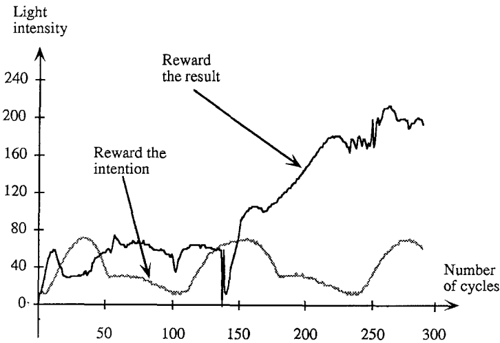
Figure 22. Difference in performance between reward-the-result and reward-the-intention training policies in the case of one blind eye.
