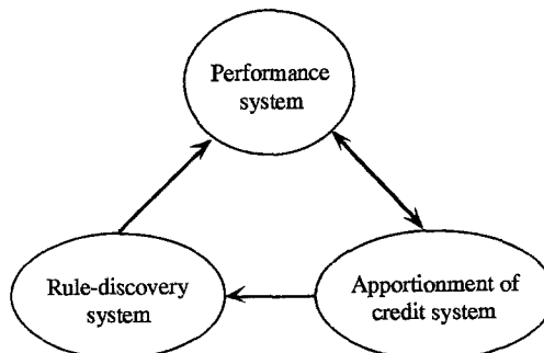
Figure 1. Functional organization of ICS.
