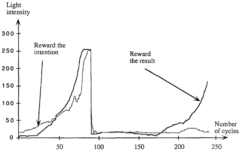
Figure 23. Difference in performance between reward-the-result and reward-the-intention training policies in the case of incorrect regulation of motors.
