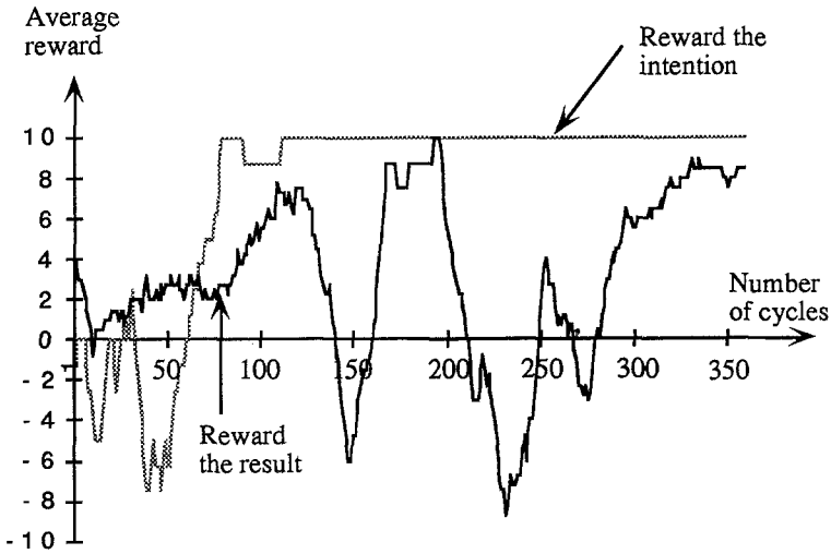
Figure 18. Difference in average reward between reward-the-result and reward-the-intention training policies.
