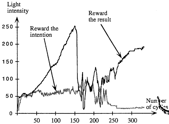
Figure 20. Difference in performance between reward-the-result and reward-the-intention training policies in the case of an AutoMouse with inverted eyes.
