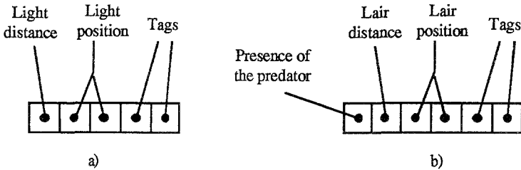
Figure 11. Structure of a message from sensory input in the case of switch architecture. a) Message going to CS-play. b) Message going to CS-hide.
