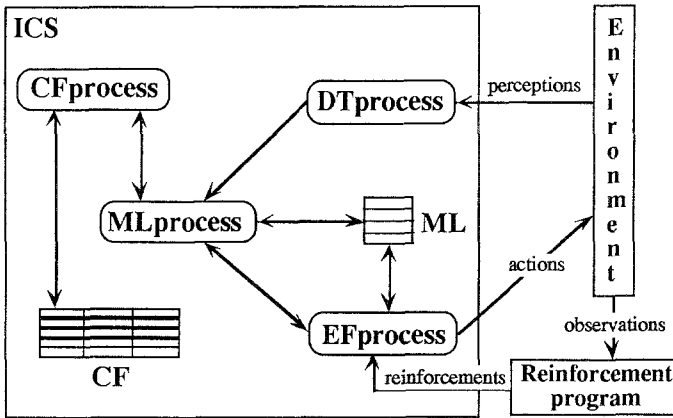
Figure 2. Concurrent processes in ICS.
