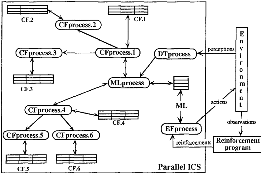
Figure 3. A parallel version of the ICS. In this example CFprocess of Fig. 2 is split into six concurrent processes CFprocess.1, ..., CFprocess.6.
